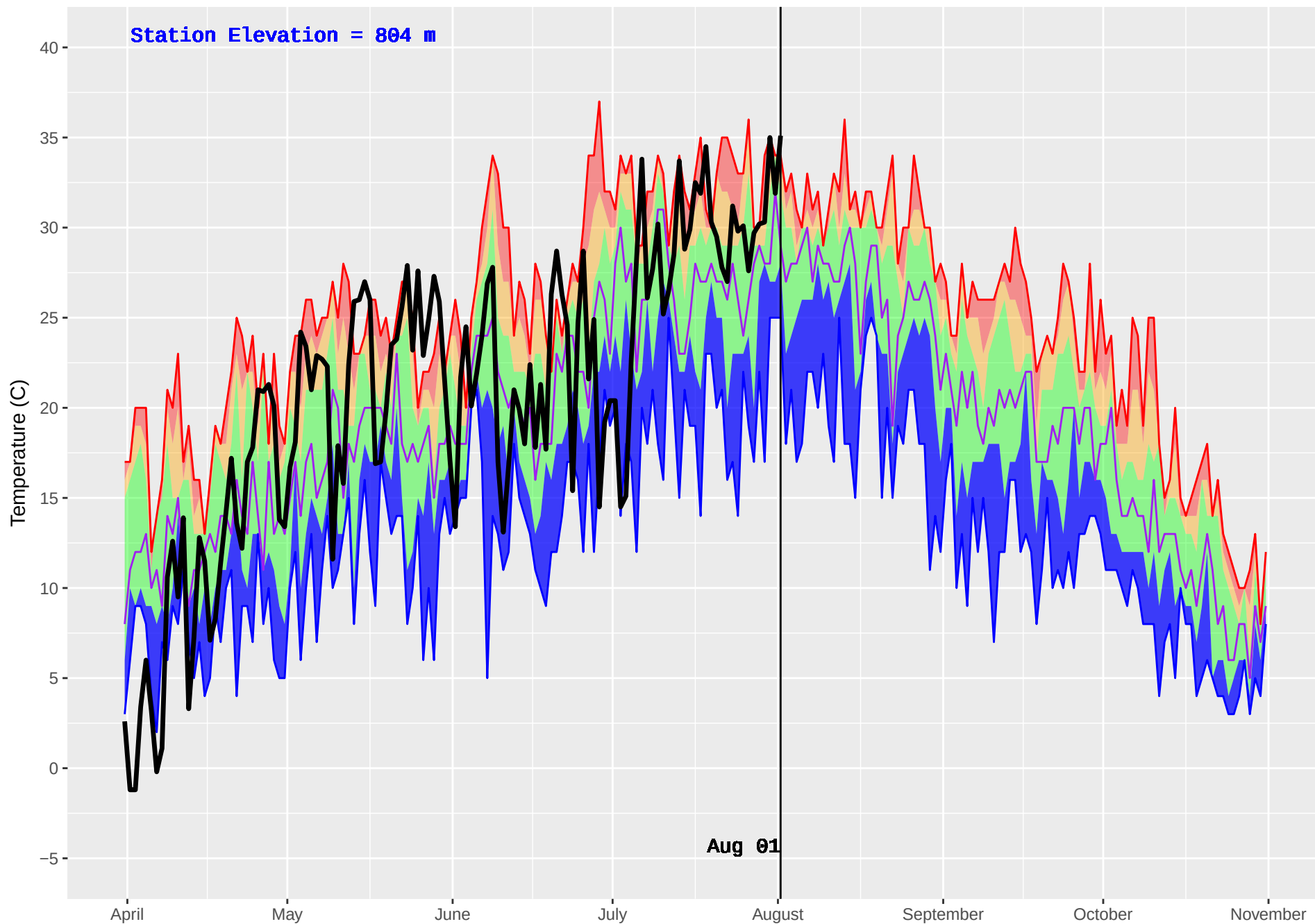
KOOCANUSA (1075) : Historical (2010–2016) and Current (2018) Daily Temperature
