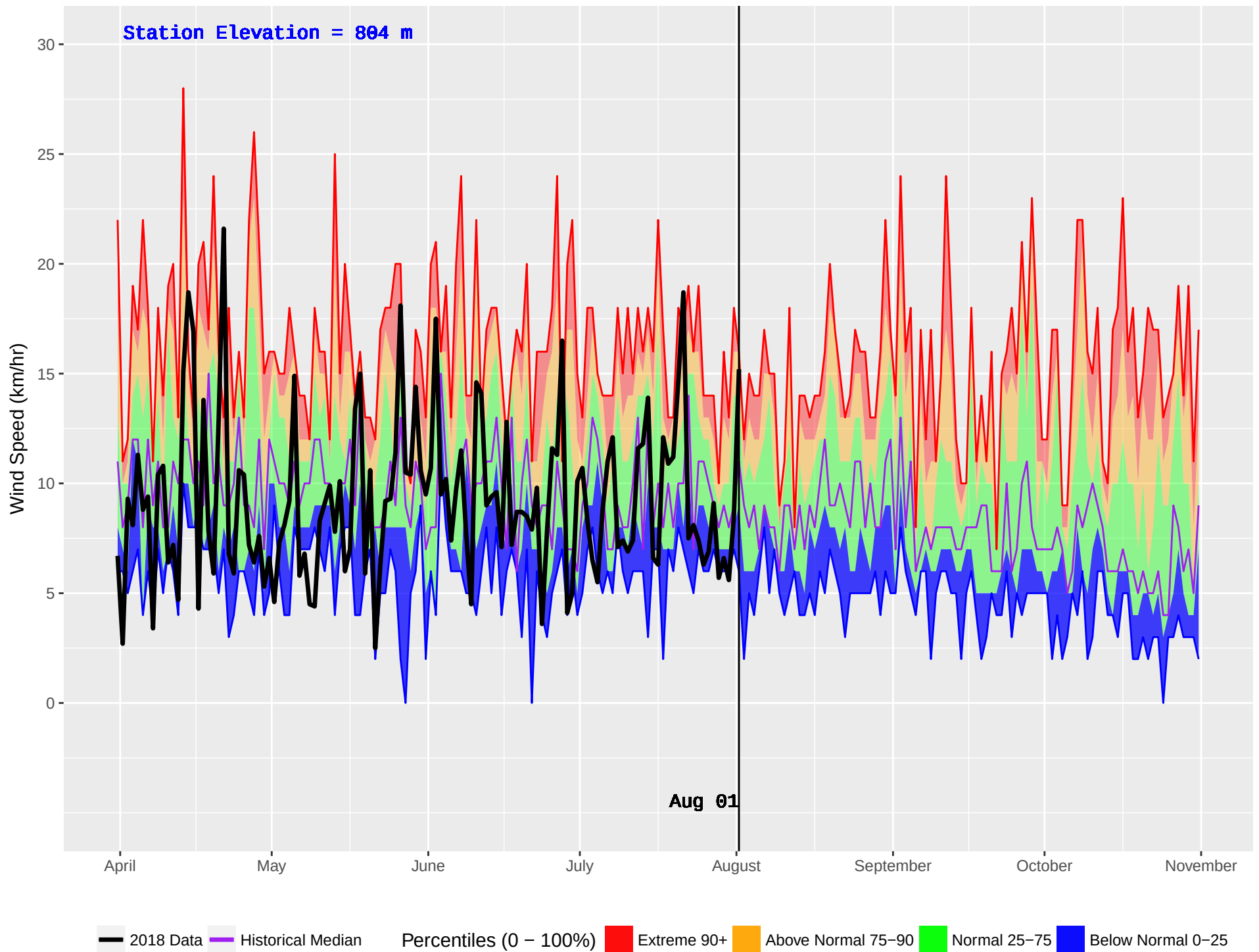
KOOCANUSA (1075) : Historical (2010–2016) and Current (2018) Daily Wind Speed
