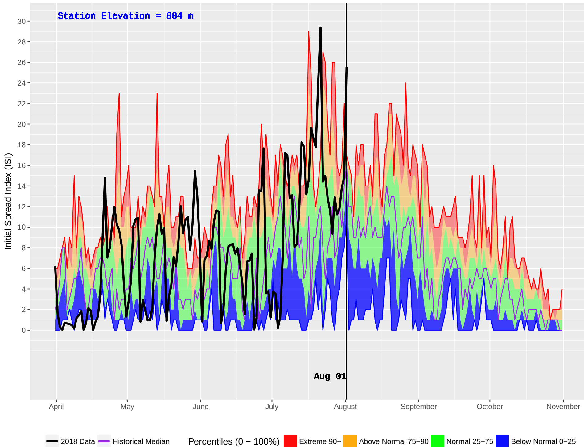
KOOCANUSA (1075) : Historical (2010–2016) and Current (2018) Daily Initial Spread Index (ISI)
