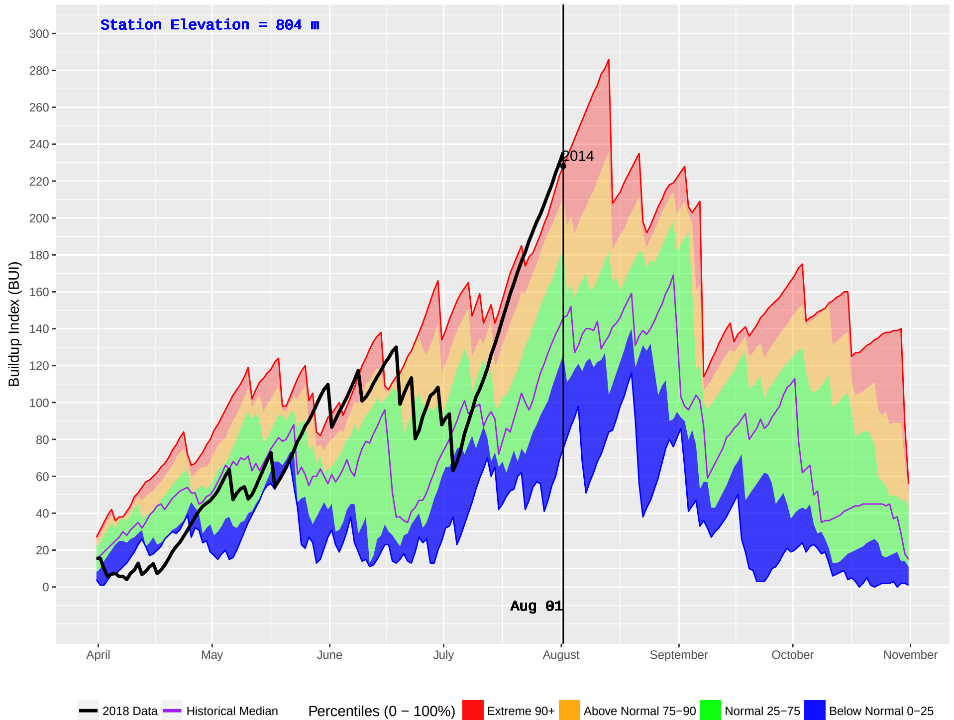
KOOCANUSA (1075) : Historical (2010–2016) and Current (2018) Daily Buildup Index (BUI)
