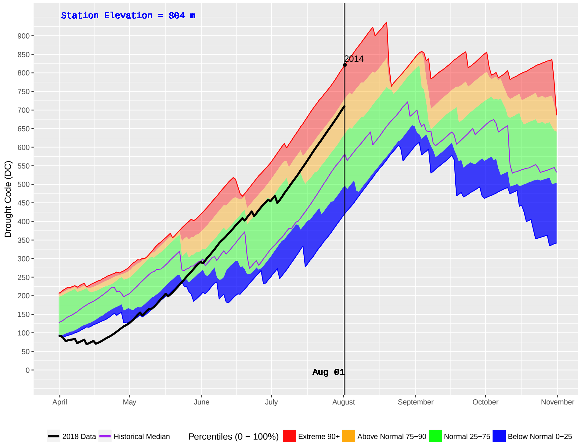
KOOCANUSA (1075) : Historical (2010–2016) and Current (2018) Daily Drought Code (DC)
